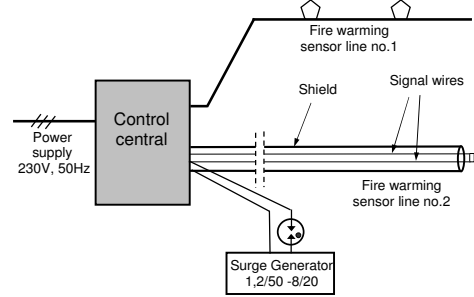
Fig. 4 – Impulse voltage between wire and shield.
