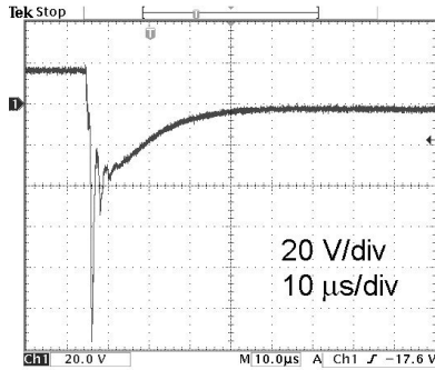
Fig. 6 - Overvoltages observed between two signal line wires caused by surge voltage 1 kV input between signal wire and shield.
