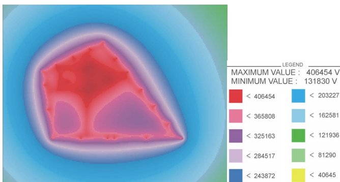
Figure 4. Contour plot of the scalar potential distribution in and around the base station
