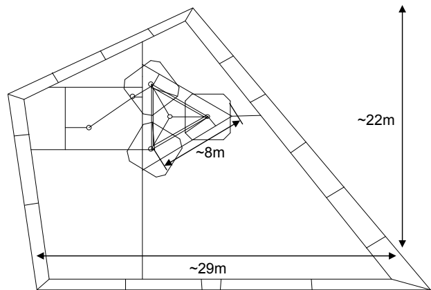
Figure 3. Thin wire model of the GSM base station – top view
