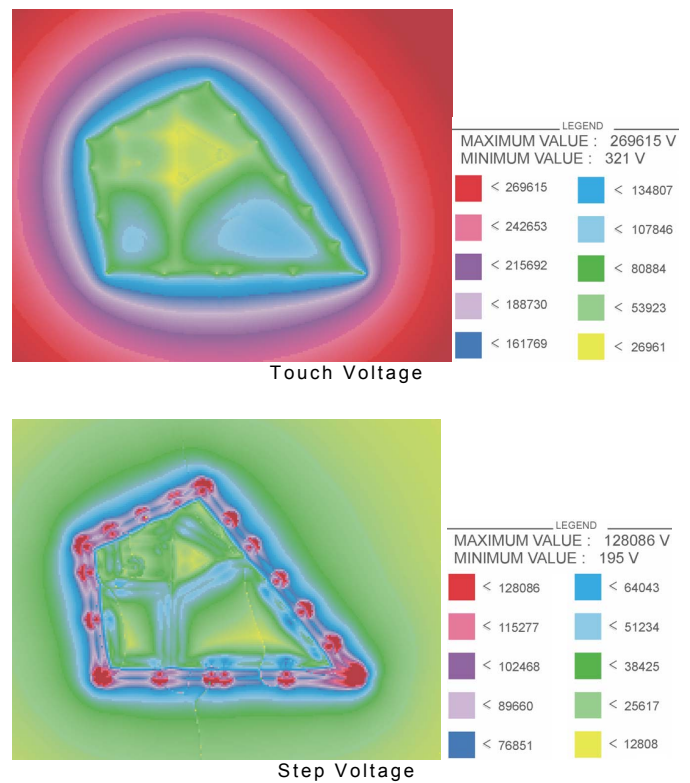
Figure 5. Touch and step voltages in and around the base station
