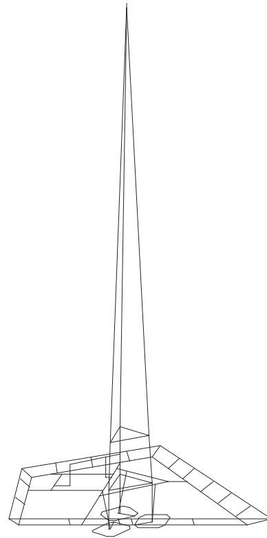
Figure 2. Thin wire model of the GSM base station – 3D view
