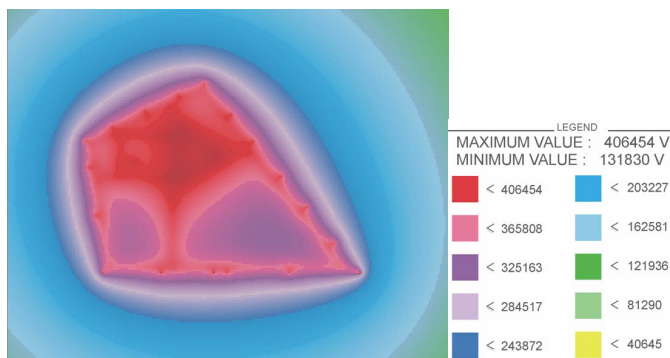
Figure 4. Contour plot of the scalar potential distribution in and around the base station
