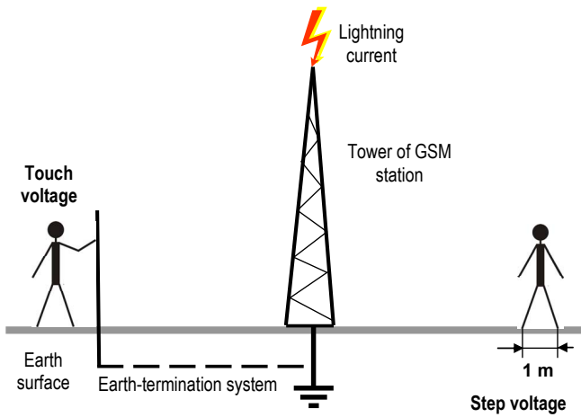
Figure 1: Transient step and touch voltages
